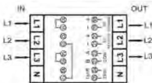
Ex9EMS 3P 4M - Direct connected - 3P 3W Open Delta (Aron)
