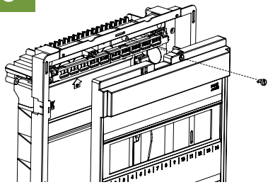
4 point connection
