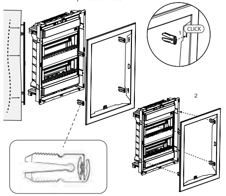
4 point connection
