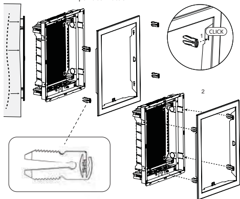
4 point connection
