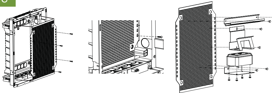
4 point connection
